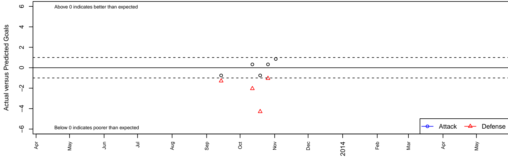
3 Rivers Flannery B98 Dots are actual minus expected GF (blue circles) and GA (red triangles). Blue line is smoothed change in attack strength. Red is smoothed change in defense strength.
